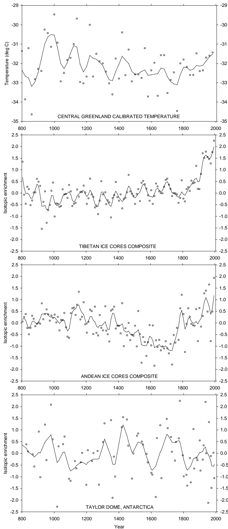
FIGURE 6-2 Two composite isotopic records from low latitudes, and two isotopic records from single locations on the polar ice sheets. Top: Record for central Greenland (GISP2 site), converted to temperature by calibration against borehole temperatures. Second from top: Composite record (normalized to mean and standard deviation) for four ice cores from Tibet. Third from top: Composite record (normalized to mean and standard deviation) for three ice cores from the equatorial Andes. Bottom: Normalized record (deuterium) from Taylor Dome, Antarctica. In each plot, data are shown as point measurements, and a smoothed version superimposed for clarity of trends. The central Greenland and Taylor Dome series are smoothed using a 100-year triangular filter, while the composite series use a 50 year triangular filter. SOURCES: Cuffey and Clow (1997), Thompson et al. (2003, in press), Steig et al. (2000).
