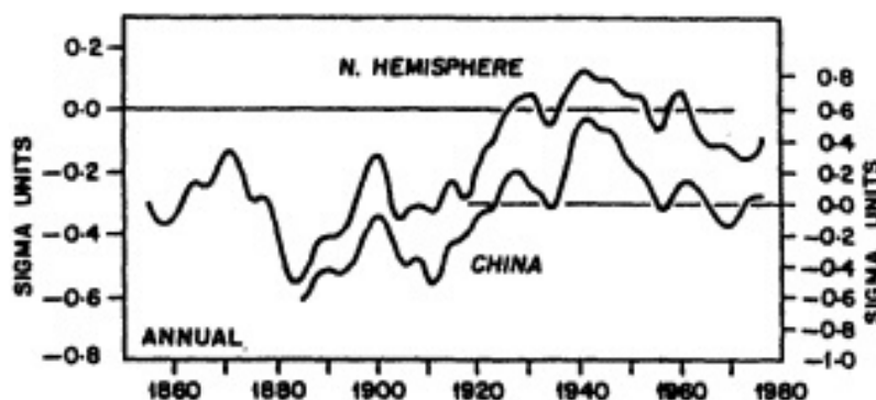
FIGURE 2-4 Smoothed time series of normalized annual mean surface air temperature averaged over China and the entire Northern Hemisphere. SOURCE: Bradley et al. (1988). Reprinted with permission, Taylor & Francis Ltd. ( http://www.tandf.co.uk/journals ), copyright 1988.
