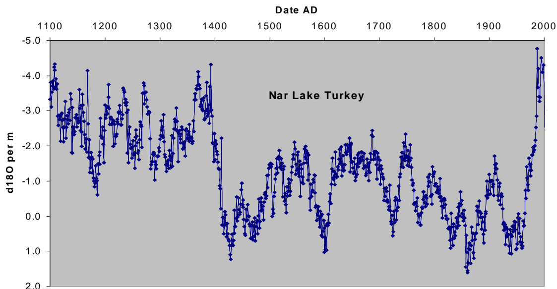
FIGURE 5-7 Annually resolved oxygen isotope record for the last 900 years from varved crater lake carbonates in the East Mediterranean. SOURCE: Jones et al. (2006).
