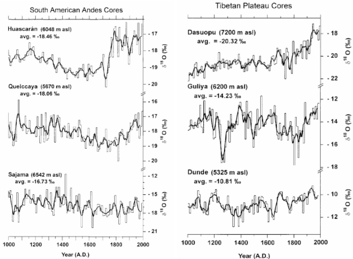
FIGURE 6-1 Isotopic records from high-altitude ice cores from the equatorial Andes (left) and the Tibetan Plateau (right). Higher isotopic values generally indicate warmer conditions, but the records from the Andes may be dominated by hydrologic factors such as precipitation in Amazonia. SOURCE: Thompson et al. (2003).
