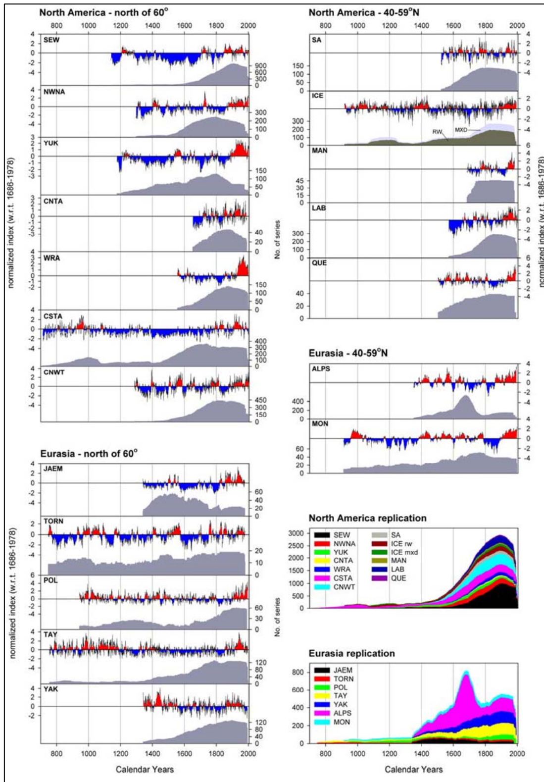
FIGURE 4-2 Results for individual regional composite chronologies for the sites shown in Figure 4-1. The time series have been loosely grouped according to latitude bands and normalized to the common period. The bottom two panels in the right column show grouped replication plots for both North America and Eurasia. SOURCE: D'Arrigo et al. (2006).
