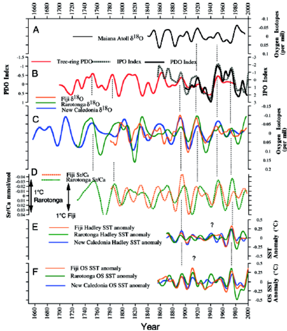
FIGURE 5-2 (A)–(F) Comparison of interdecadal variability in geochemical records from Porites corals from Rarotonga (Linsley et al. 2000), Fiji and New Caledonia (Quinn et al. 1998), and Maiana Atoll (Urban et al. 2000). The long-term trend has been removed from all data; thus, the warming during the 20th century cannot be seen. Also shown are instrumentally based indices of the Interdecadal Pacific Oscillation (IPO) (Folland et al. 2002a) and Pacific Decadal Oscillation (PDO) (Mantua et al. 1997) indices, along with the North American tree-ring-based PDO index of D’Arrigo et al. (2001) and SST data from Rarotonga, Fiji, and New Caledonia from two different datasets (HADISST1 and Kaplan et al. [1998]). SOURCE: Linsley et al. (2004).
