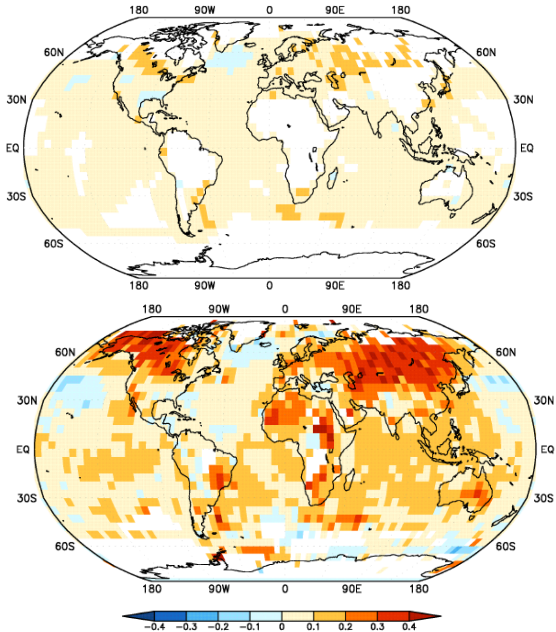
FIGURE 2-3 Observed surface temperature trends in degrees Centigrade per decade through 2005 beginning in 1870 (top) and beginning in 1950 (bottom) derived from HadCRUT2v data. SOURCE: Data from Jones et al. (2001); drawing by Todd Mitchell, University of Washington, Seattle.
