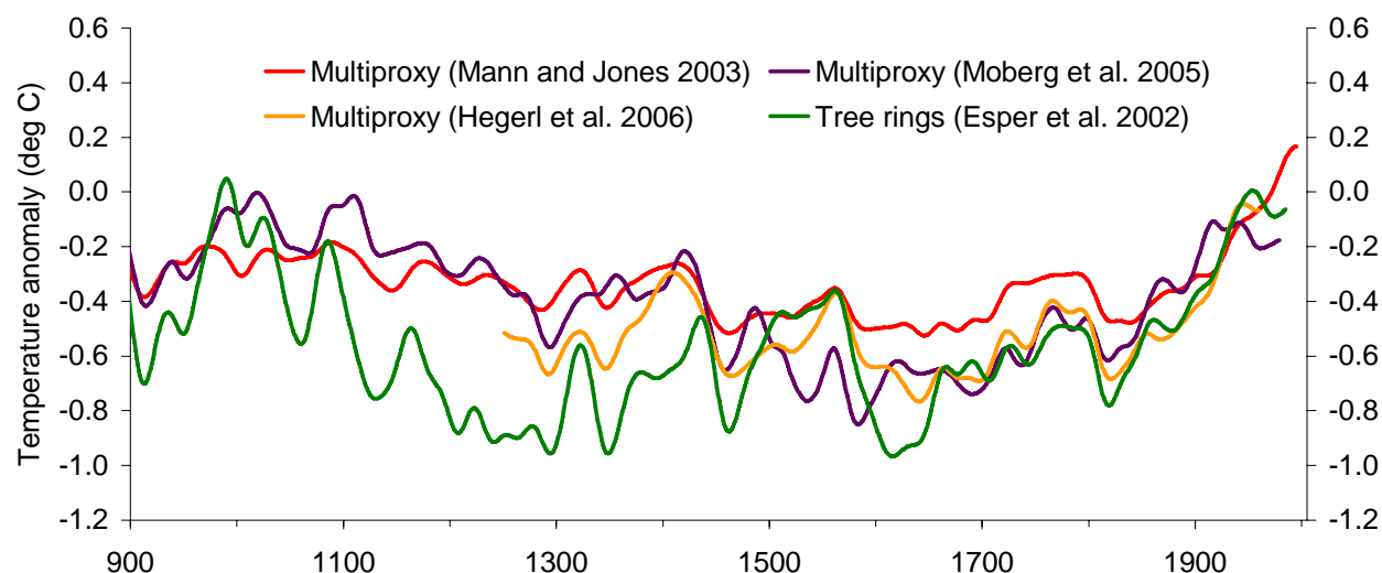
FIGURE 11-1 Four different large-scale multiproxy- and tree-ring-based surface temperature reconstructions, shown for the period A.D. 900–2005. See Figure O-5 for additional information on each data series.
