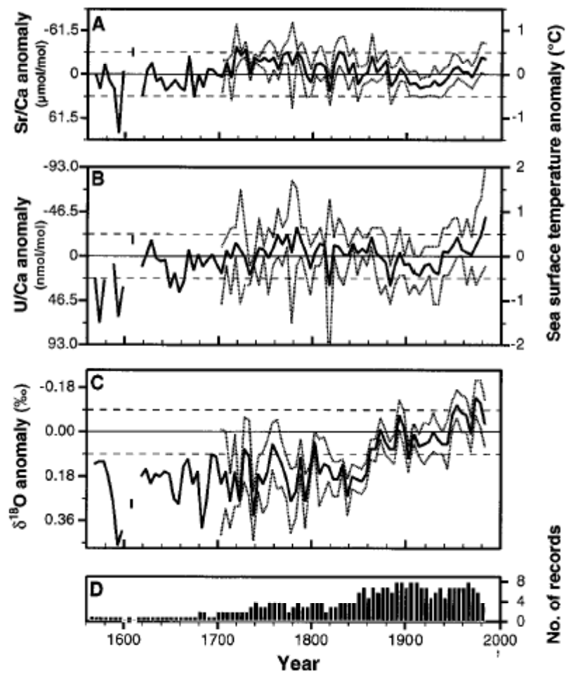
FIGURE 5-1 Sr/Ca, U/Ca, and \delta^{18}\text{O} anomalies from Great Barrier Reef composites; the Sr/Ca and U/Ca anomalies have been used to reconstruct local SST records for five-year averages, with 95 percent statistical confidence intervals indicated by dotted lines. SOURCE: Hendy et al. (2002).
