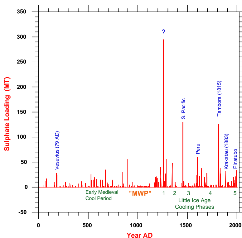
FIGURE 10-3 Ice core estimates of global stratospheric sulfate loading from volcanoes (A.D. 1-2005). SOURCE: Hegerl (2006).
