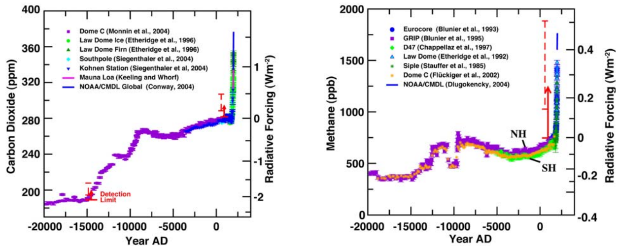
FIGURE 10-1 Evolution of atmospheric carbon dioxide and methane over the last 22,000 years. Left-hand axes show atmospheric concentrations (note the carbon dioxide scale does not start from zero) and right-hand axes show the radiative forcing relative to 1750 as calculated using the formulas given by Myhre et al. (1998) and Ramaswamy et al. (2001). Red arrows indicate the theoretical detection limit of a forcing (relative to Last Glacial Maximum and preindustrial conditions) within a climate system model, assuming an internal climate variability or detection threshold of 0.2^{\circ}\text{C} , climate equilibrium, and a mid-range climate sensitivity of 3^{\circ}\text{C} for a carbon dioxide doubling. Dashed red lines indicate the uncertainty of the detection threshold associated with the climate sensitivity range of 1.5 to 4.5^{\circ}\text{C} . SOURCE: Joos (2005).
