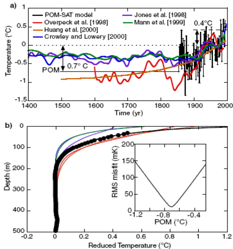
FIGURE 8-2 Here, six climate reconstructions have been used to predict ground subsurface temperature. For each curve in the upper panel, the temperature reconstruction is used as the surface temperature for a thermal model to predict the temperature at depth. The top panel shows the six reconstructions, with zero defined as the 1961–1990 mean. The reconstruction shown in black (labeled POM-SAT) uses the borehole temperatures to constrain the Pre-Observational Mean (POM) and uses the instrumental temperature record from 1856 onward. The measured subsurface temperature pattern (bottom panel, black circles) is explained almost perfectly by the instrumental record and preceding cool centuries (black curve in the top panel). SOURCE: Harris and Chapman (2001).
