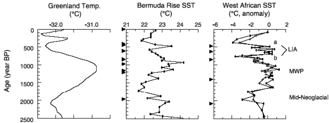
FIGURE 5-5 Greenland temperature (Dahl-Jensen et al. 1998), Bermuda Rise SST (Keigwin 1996), and West African SST for the last 2,500 years. SOURCE: deMenocal et al. (2000).
