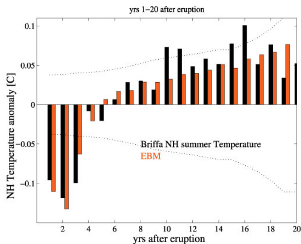
FIGURE 10-5 Comparison of the average response to volcanic eruptions in an energy balance model and the Briffa et al. (2001) reconstruction for the year of the eruption (year 1) to the next major eruption. Dotted lines represent 9–95 percent uncertainty ranges for the observed response (note the sample size decreases with time). SOURCE: Hegerl et al. (2003).
