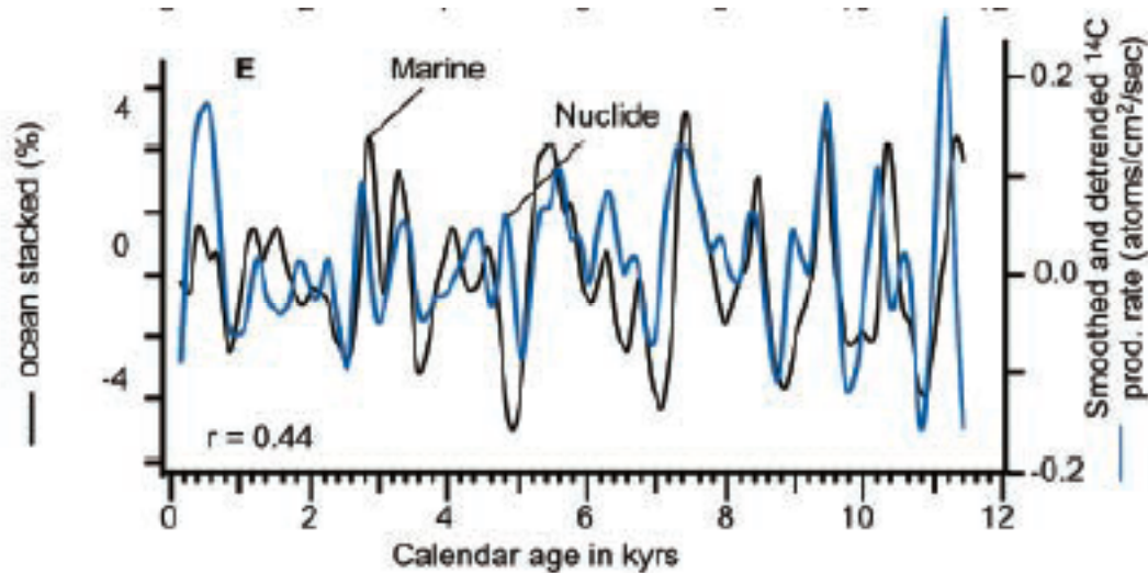
FIGURE 5-6 Relationship between the concentration of ice-rafted debris (as inferred from iron [Fe] concentration) and the flux of cosmogenic ^{14}\text{C} . SOURCE: Bond et al. (2001).
