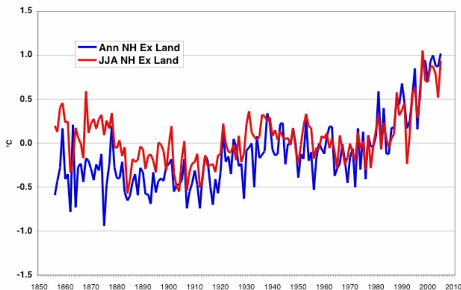
FIGURE 2-2 Annual mean and summer (June–August) mean temperature anomalies for Northern Hemisphere extratropical land areas from the HadCRUT2v surface temperature dataset. SOURCE: Jones et al. (2001).
